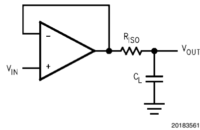
FIGURE 1. Isolation of C_{\text{L}} to Improve Stability
